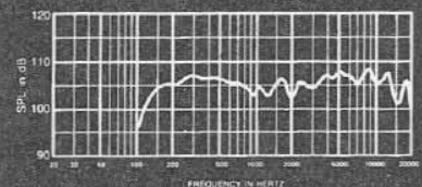
FIGURE 1 Axial Frequency Response using Recommended Crossover, Equalization 1 Watt/1 Meter into MB Section
